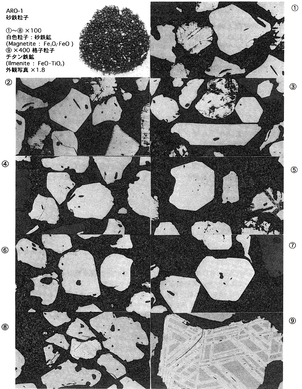
PHOTO.1 砂鉄の顕微鏡組織 (荒尾市関川、岩本橋周辺) Microscopic organization of iron sand
